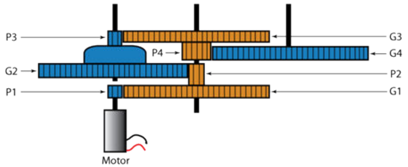
Futaba S3003 standard servo gear train
